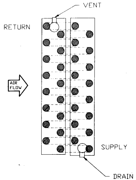
DOUBLE CIRCUIT (00)
