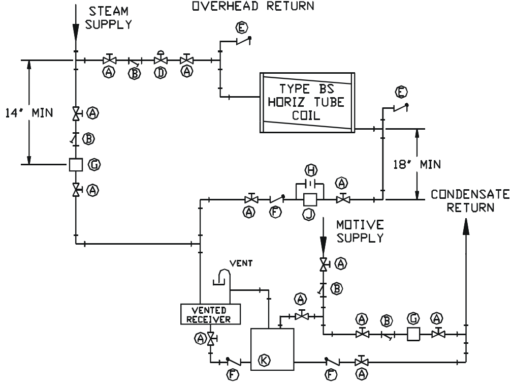
FIGURE 6 PROCESS HEATING SYSTEM PIPING MODULATING SUPPLY VALVE OVERHEAD RETURN
