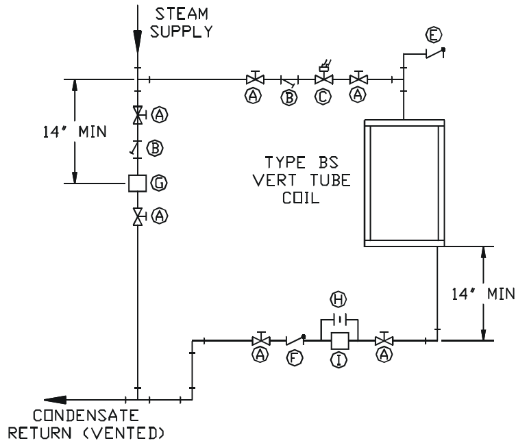
FIGURE 2 PREHEAT SYSTEM PIPING NON-MODULATING SUPPLY VALVE VENTED RETURN
