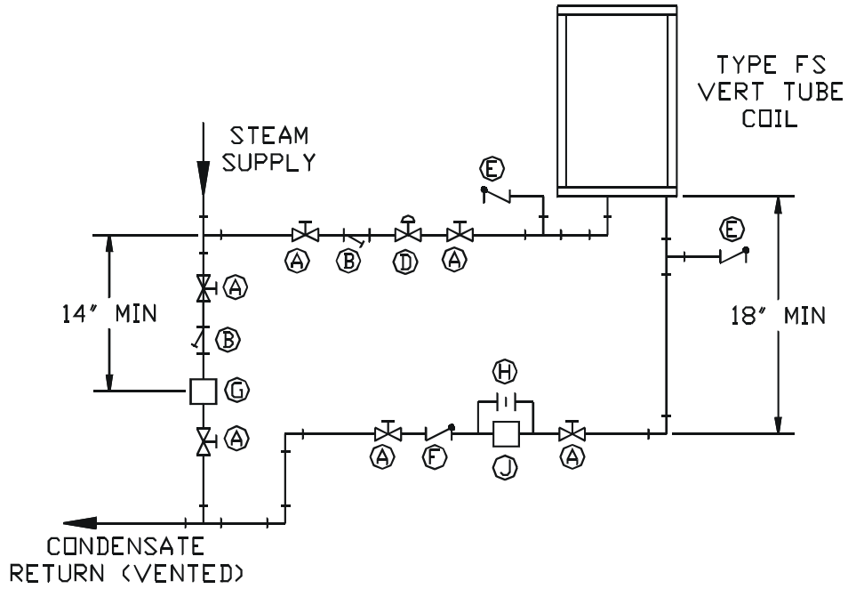
FIGURE 4 REHEAT SYSTEM PIPING MODULATING SUPPLY VALVE VENTED RETURN
