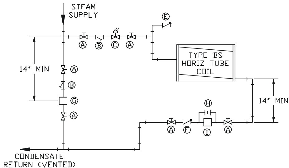
FIGURE 1 PREHEAT SYSTEM PIPING NON-MODULATING SUPPLY VALVE VENTED RETURN
