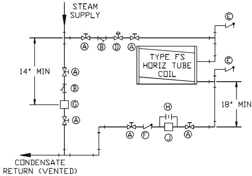
FIGURE 3 REHEAT SYSTEM PIPING MODULATING SUPPLY VALVE VENTED RETURN
